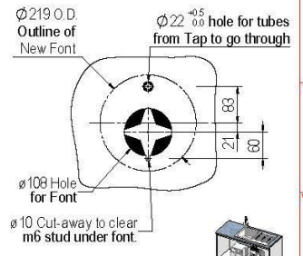
DETAIL FONT SCALE 1:5
