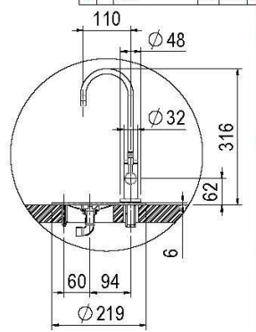
DETAIL FONT SCALE 1:5
